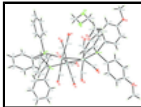
Fig. 1. The molecular structure of the title compound with 30% probability ellipsoids for non-H atoms. Atoms with suffix A are generated by the symmetry operation (1 - x, 1 - y, 1 - z) .
